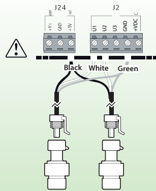
Ratiometric Probe:
